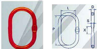
Argolão oval especial Special oblong masterlink
